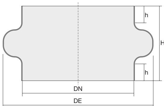
Compensatore a onda in silicone trasparente Wave Compensator made with transparent silicone
