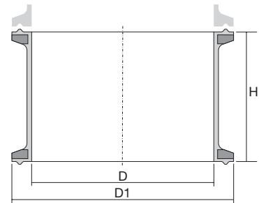
C-T.C. 4" SI-B - Silicone conforme F.D.A. C-T.C. 4" SI-B - Silicone in compliance with F.D.A. requirements
